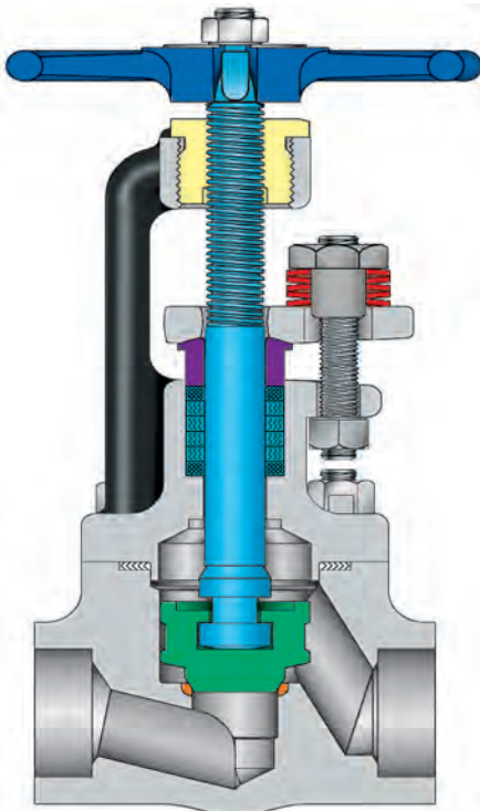
GLOBE VALVE
