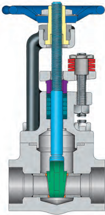
GATE VALVE
