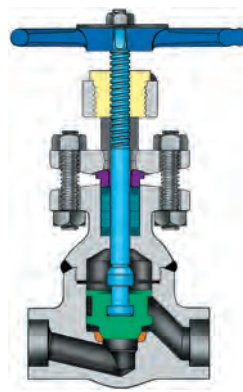
WELDED BONNET 2074W – Class 800 3074W – Class 1500
