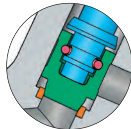
Solid CoCr alloy disc for all y-pattern valves
