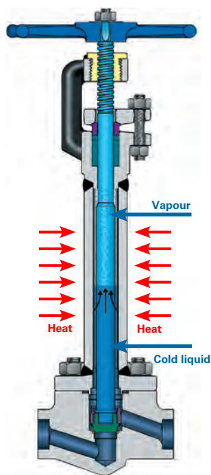
GLOBE VALVE
