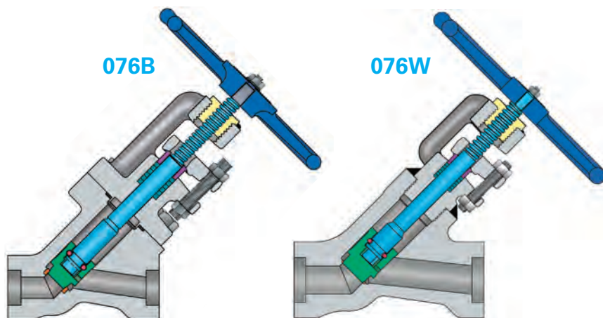
45° BOLTED BONNET
