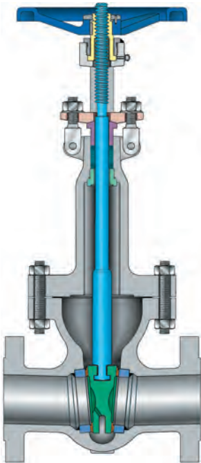
GATE VALVE
