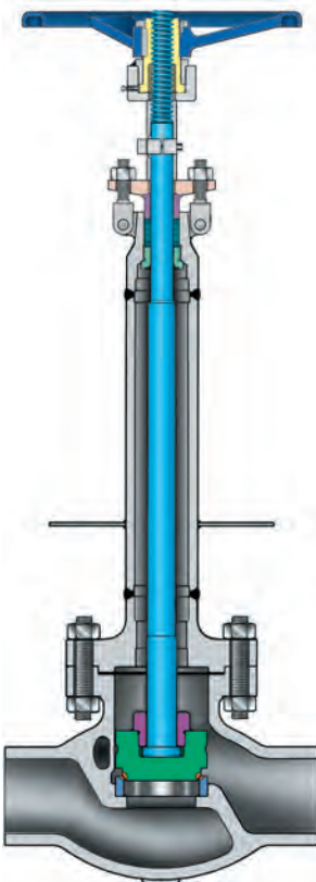
GLOBE VALVE
