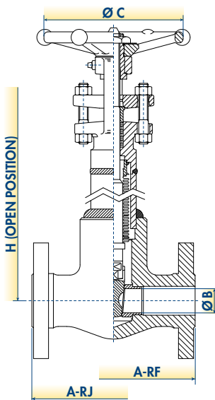
DESIGN TYPE P1 HANDWHEEL OPERATED
